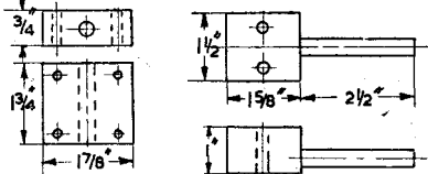
PIVOTING COUNTERSHAFT PLATE & PARTS
