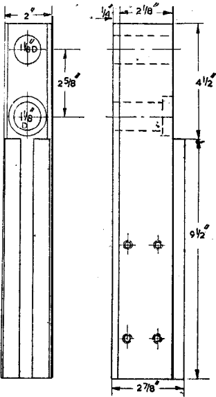
COLUMN
