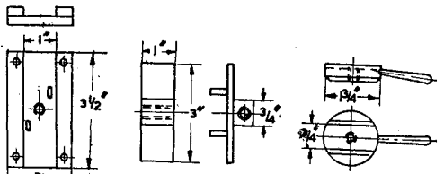
CLASP NUT & CAM ASSEMBLY
