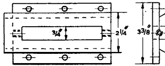
CROSS TRAVERSE LOWER SLIDE
