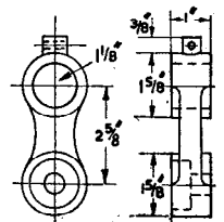
OVERARM BRACKET
