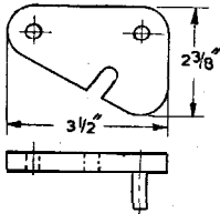
BACKGEAR QUADRANT
